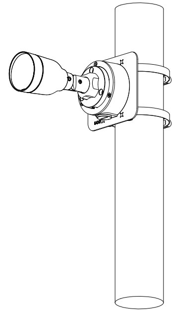
Pole Mount(Vertical)
