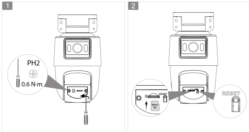
Figure 3-3 Install the SD card
