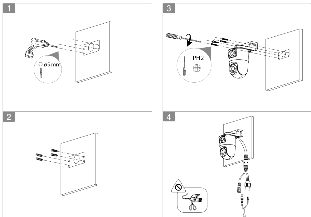
Figure 3-4 Wall mount
