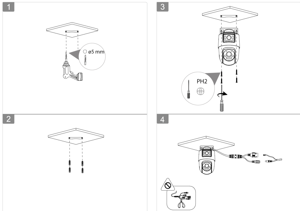
Figure 3-5 Ceiling mount
